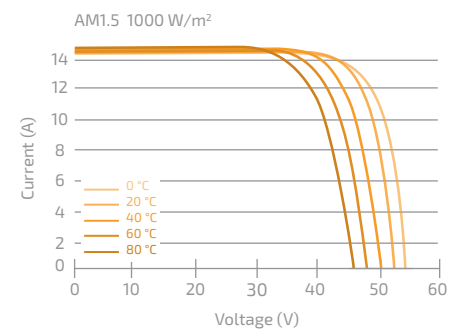
IV Curves for Front-Side Illumination of 580 Wp Panel
